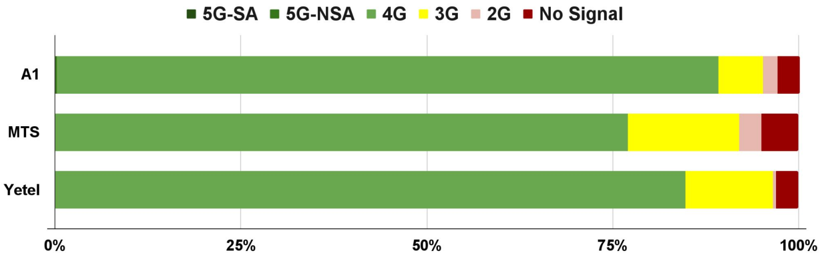
Chart 5 - Serbia: Mobile Traffic Percentage by MNO and Network Type
