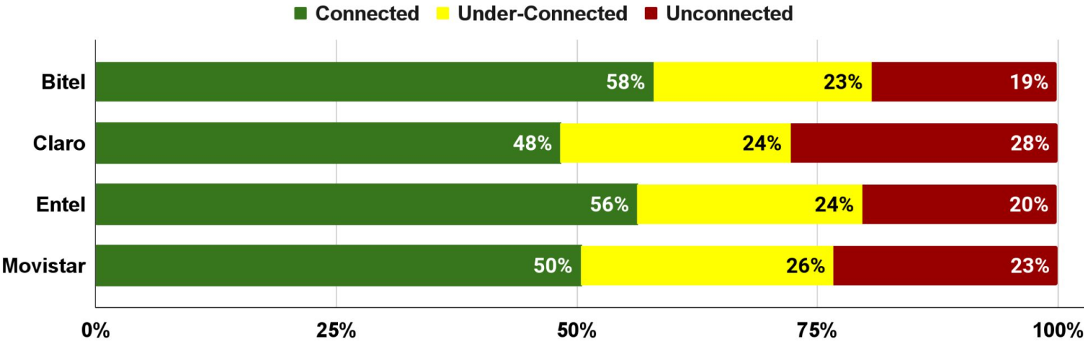
Chart 2 - Peru: Coverage-QoE by MNO
