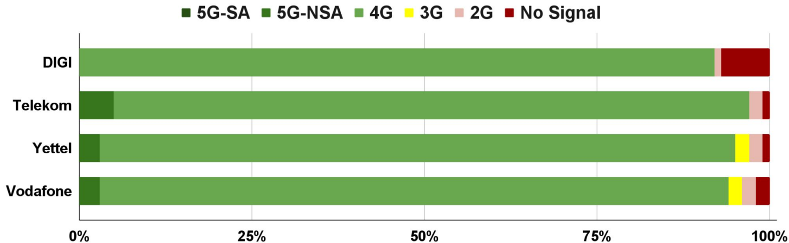
Chart 5 - Hungary: Mobile Traffic Percentage by MNO and Network Type
