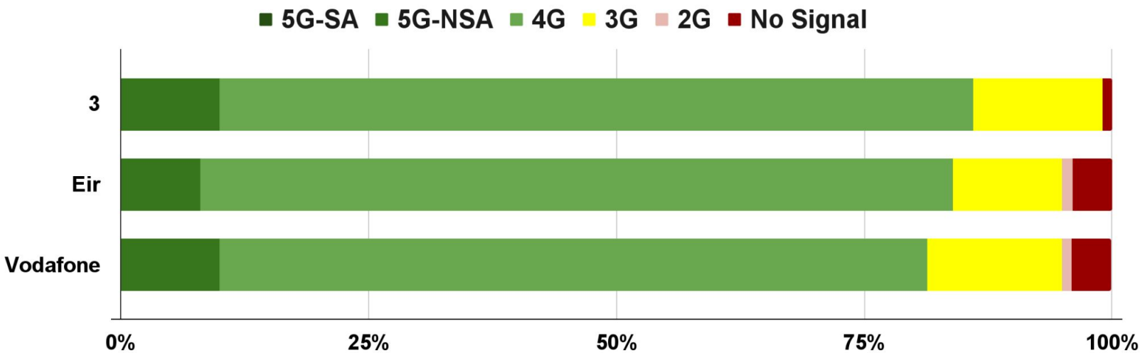
Chart 5 - Ireland: Mobile Traffic Percentage by MNO and Network Type
