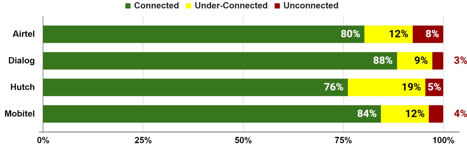
Chart 2 - Sri Lanka: Coverage-QoE by MNO
