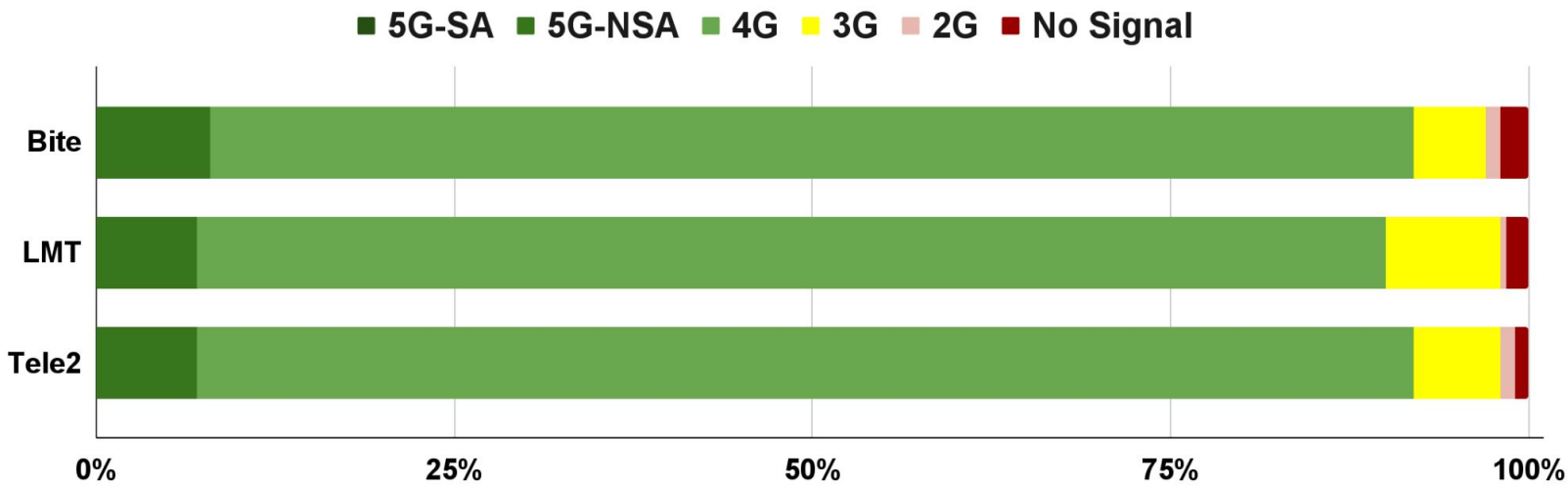
Chart 5 - Latvia: Mobile Traffic Percentage by MNO and Network Type
