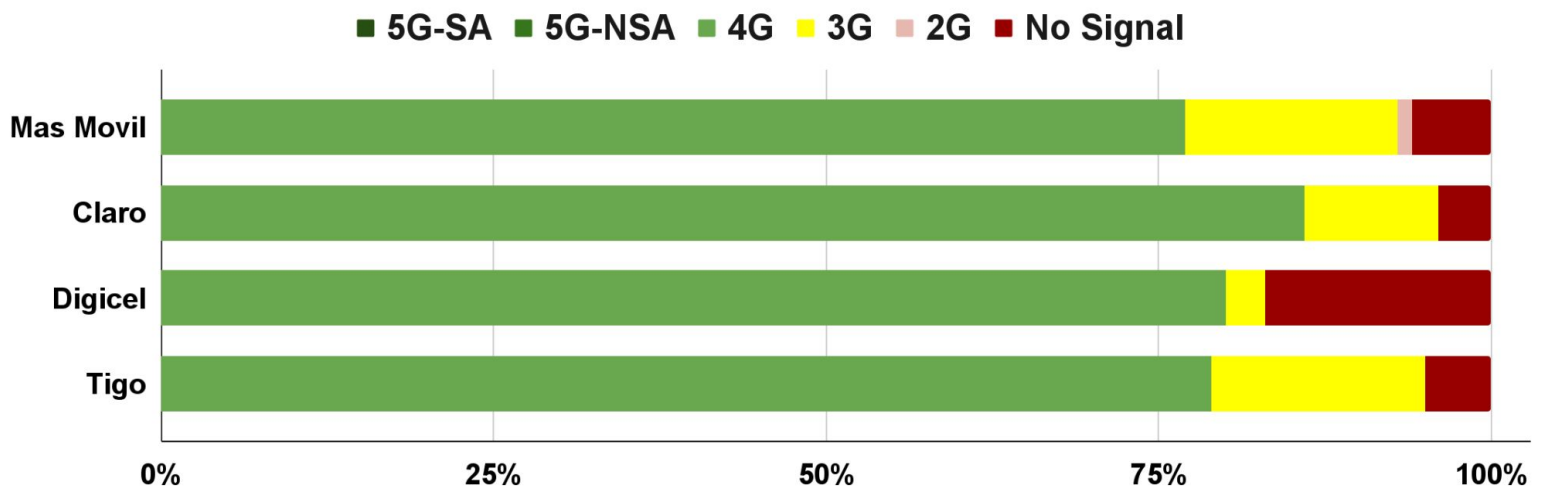
Chart 5 - Panama: Mobile Traffic Percentage by MNO and Network Type
