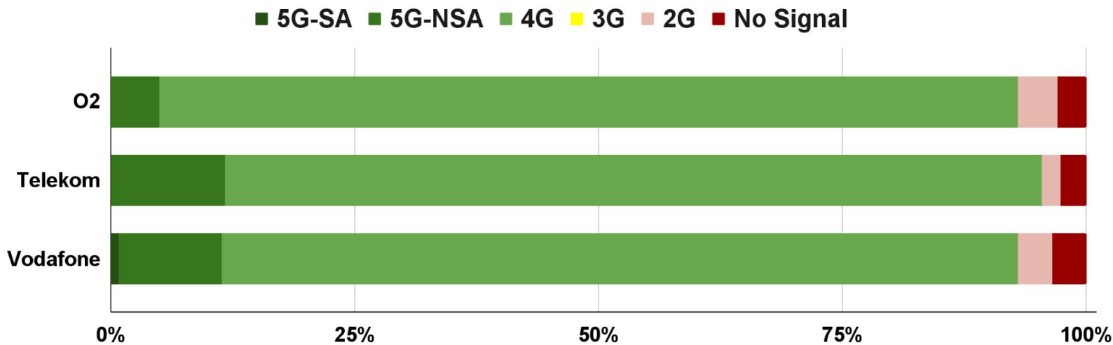
Chart 5 - Germany: Mobile Traffic Percentage by MNO and Network Type
